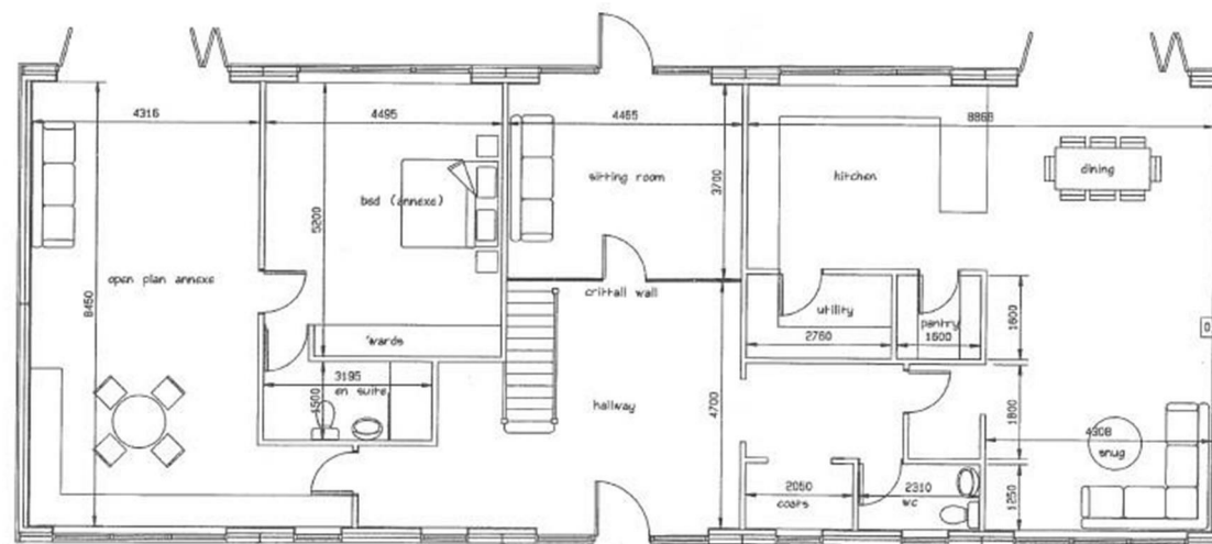
Proposed Ground Floor Plan 1:50
